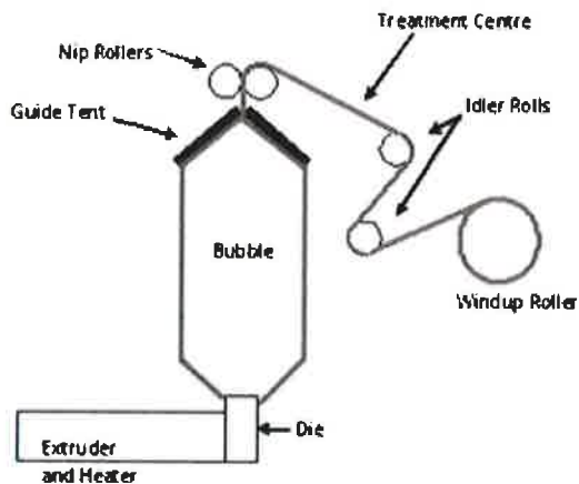
Figure 2: Blown film moulder
